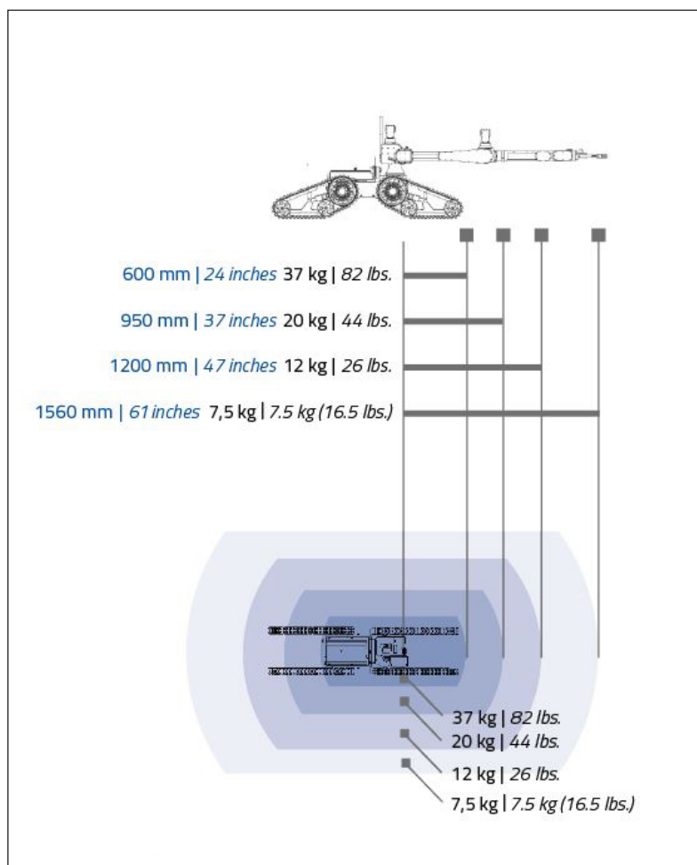
Figure: Load diagram
