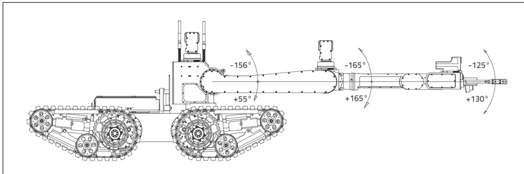
Figure: Range of movement of manipulator
