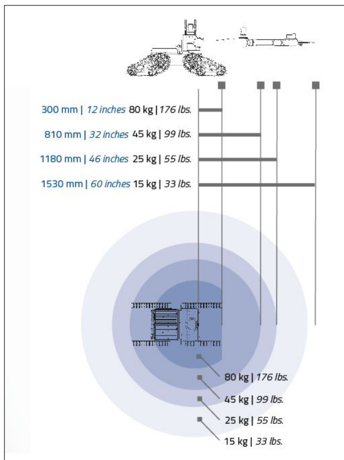
Figure: Load diagram
