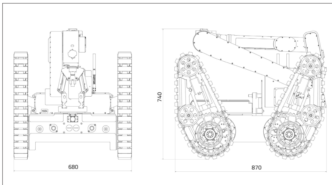
Figure: Packing position
