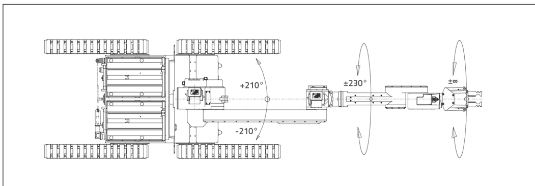
Figure: Range of movement of turret
